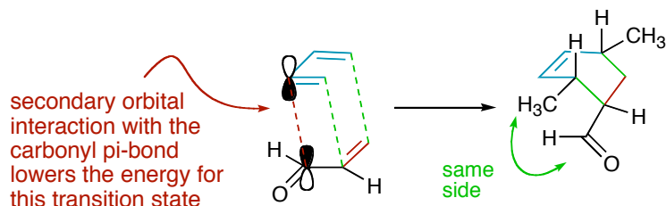
endo transition state
