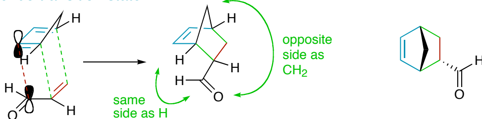
endo transition state
