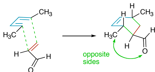
exo transition state
